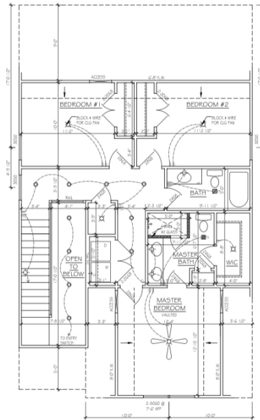
SECOND FLOOR PLAN SCALE: 1/4" = 1'-0"
